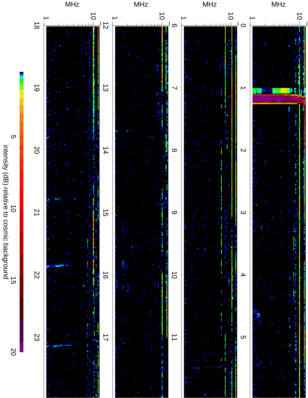
Wind Waves RAD2 receiver: 2010/06/07
