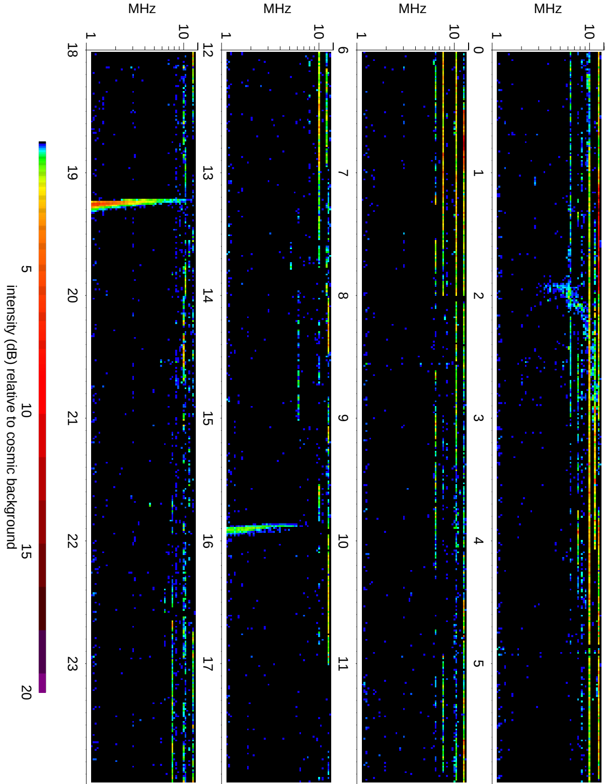
Wind Waves RAD2 receiver: 2010/06/28
