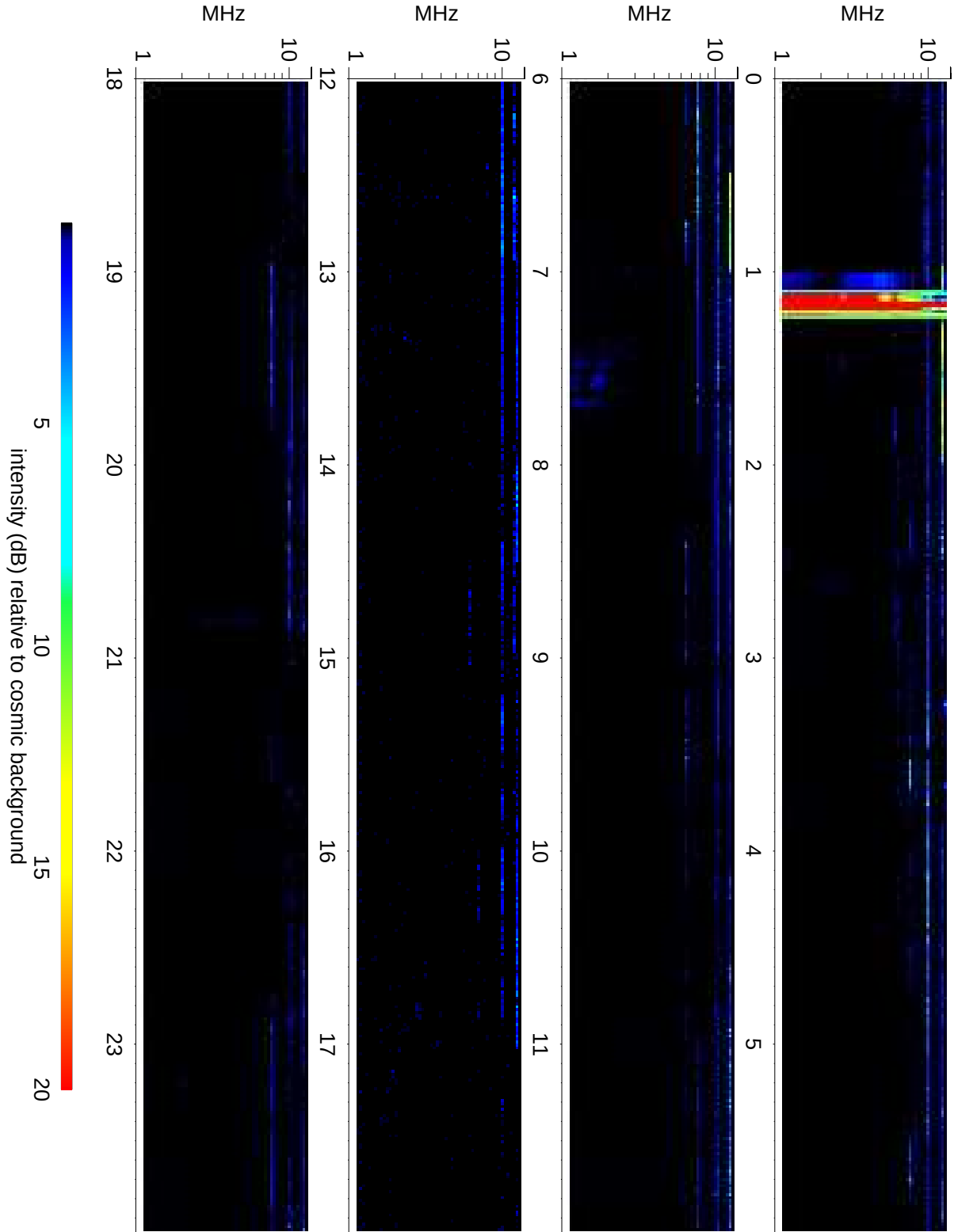
Wind Waves RAD2 receiver: 2010/07/09
