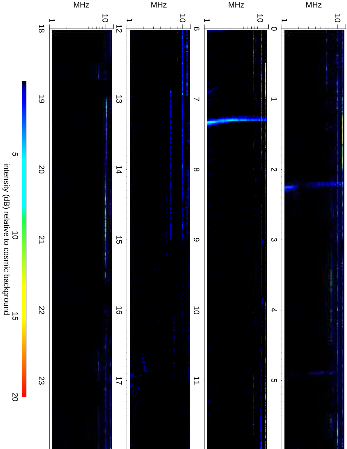
Wind Waves RAD2 receiver: 2010/07/20
