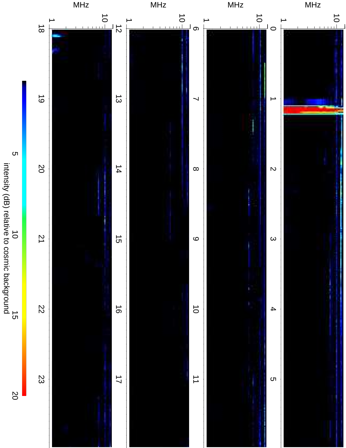
Wind Waves RAD2 receiver: 2010/07/21
