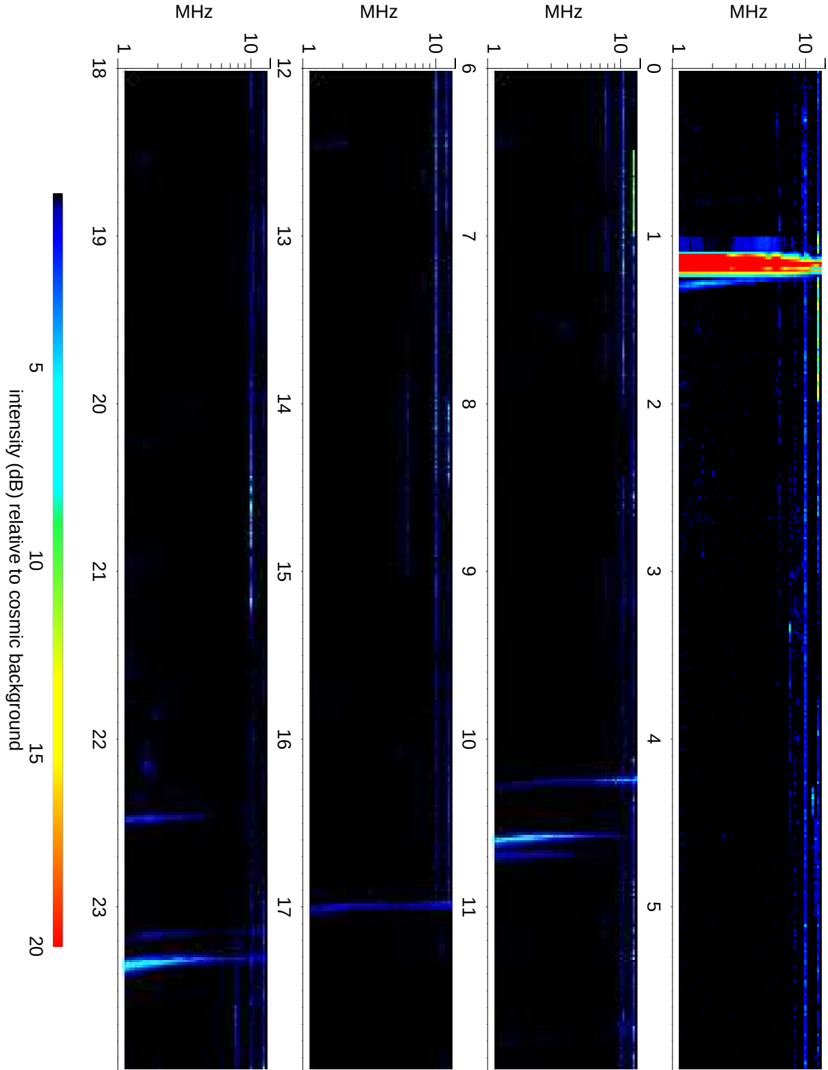
Wind Waves RAD2 receiver: 2010/07/27
