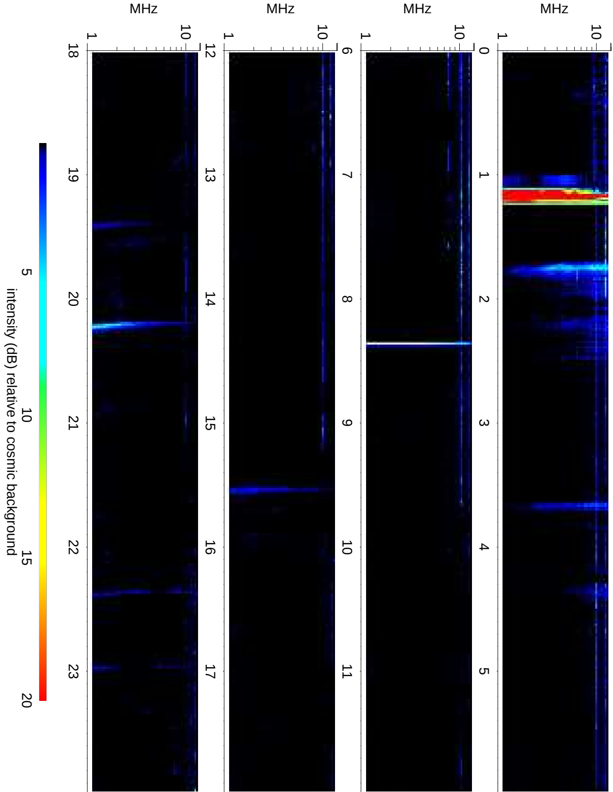
Wind Waves RAD2 receiver: 2010/08/08
