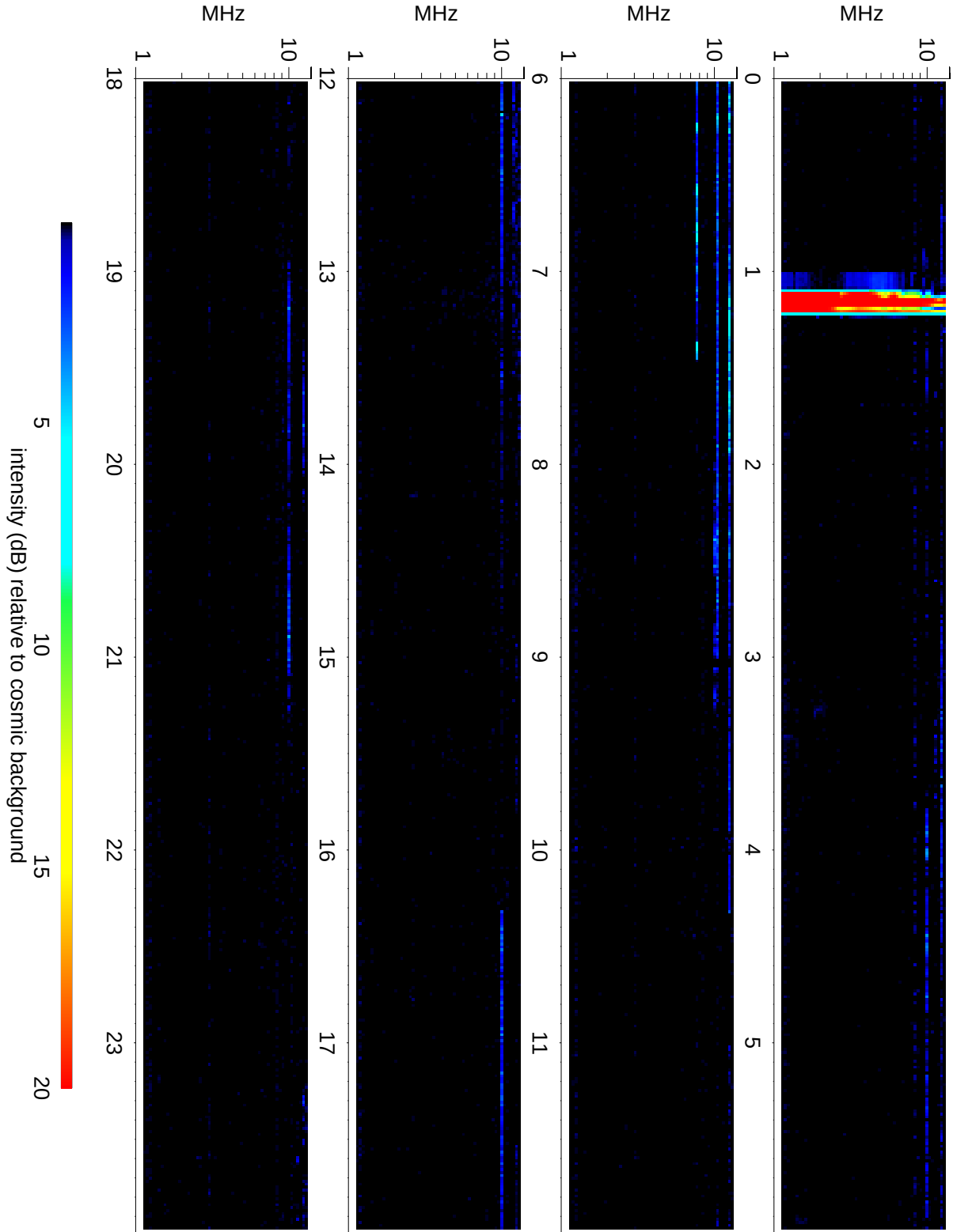
Wind Waves RAD2 receiver: 2010/08/28
