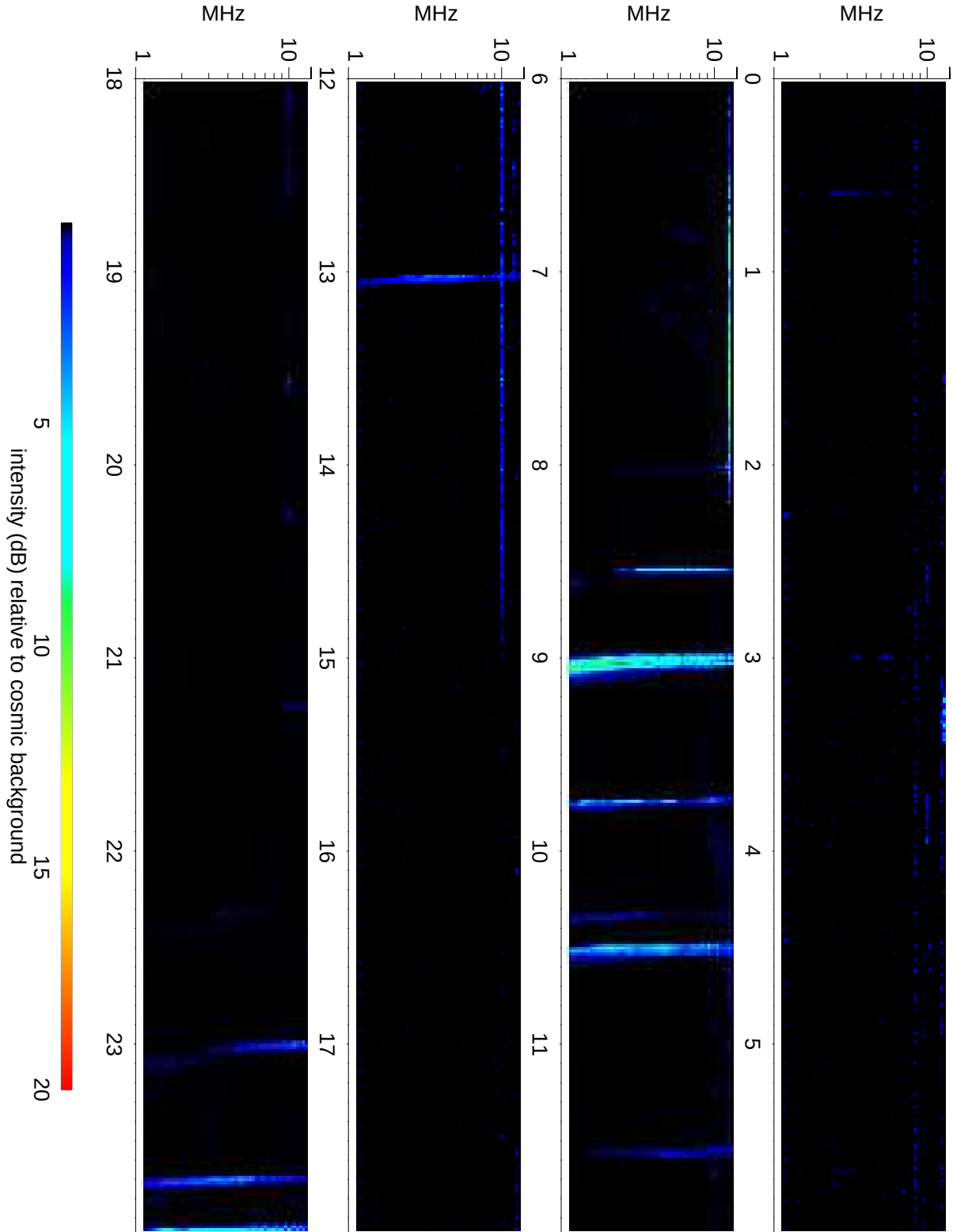
Wind Waves RAD2 receiver: 2010/09/16
