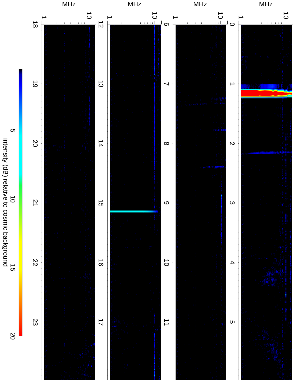
Wind Waves RAD2 receiver: 2010/09/19
