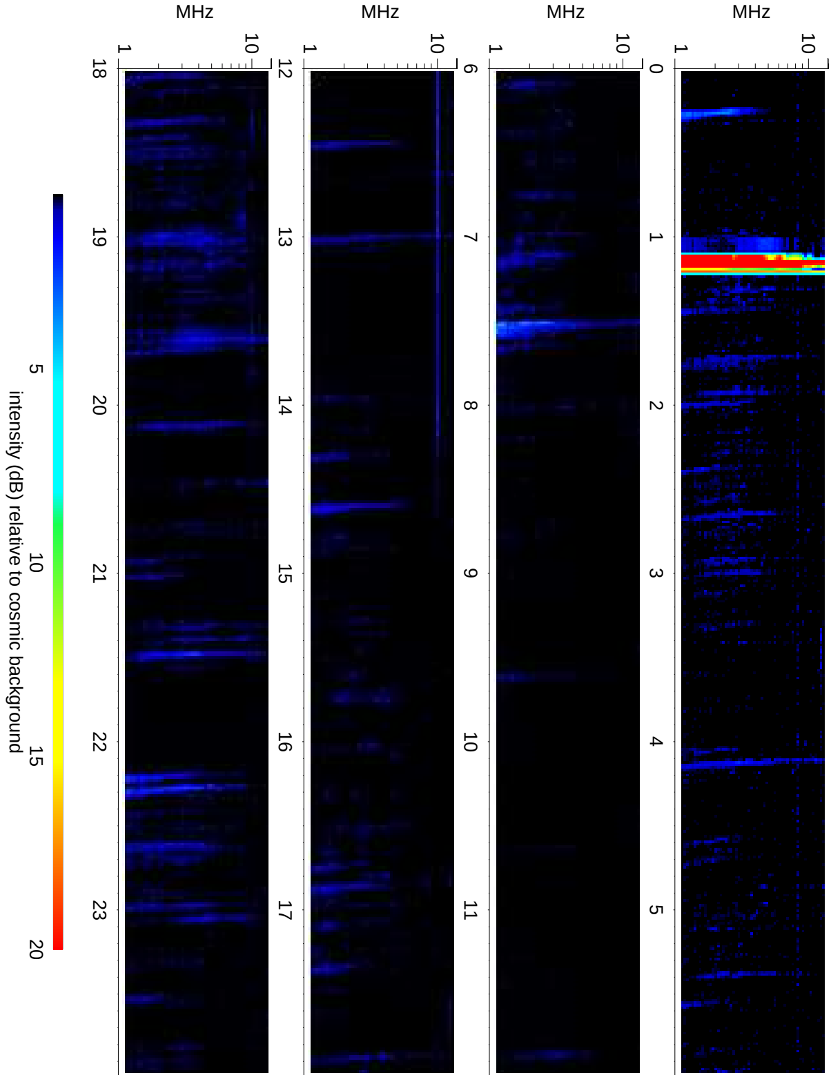
Wind Waves RAD2 receiver: 2010/09/21
