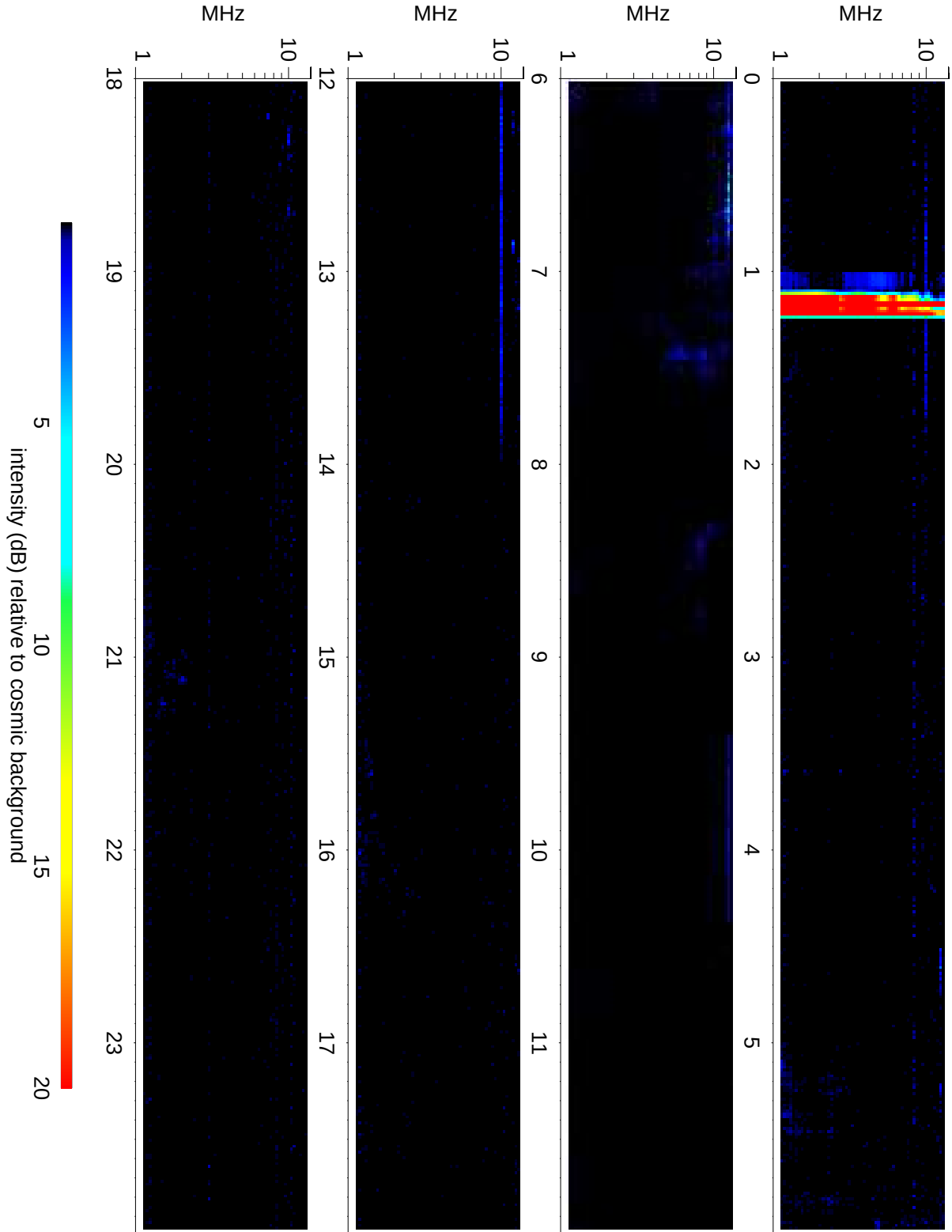
Wind Waves RAD2 receiver: 2010/09/25
