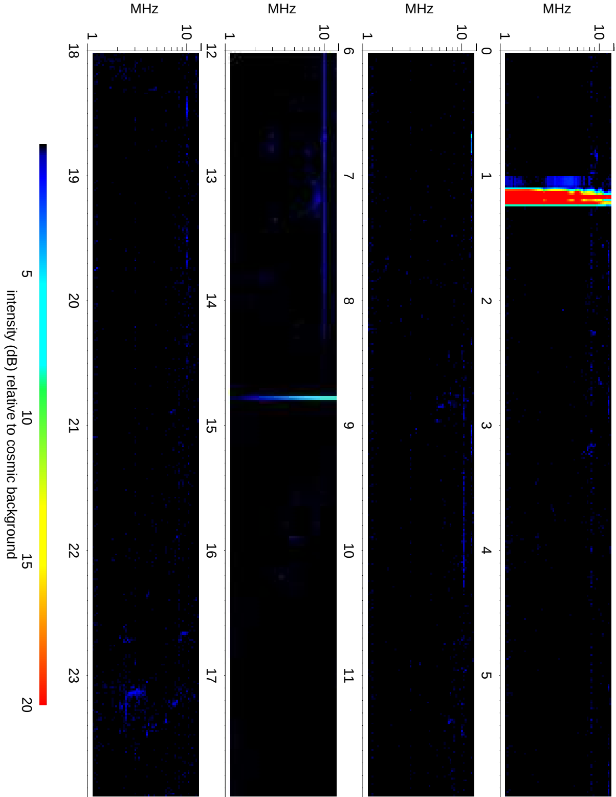
Wind Waves RAD2 receiver: 2010/10/03
