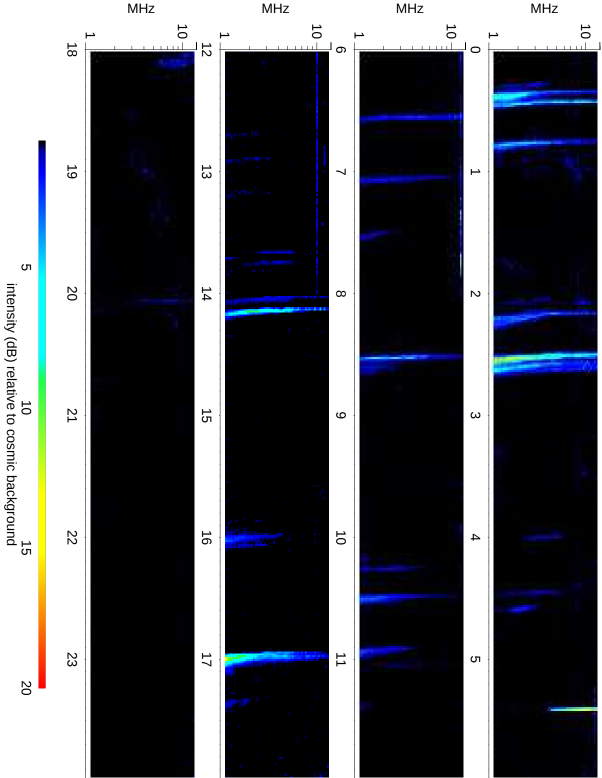
Wind Waves RAD2 receiver: 2010/10/14
