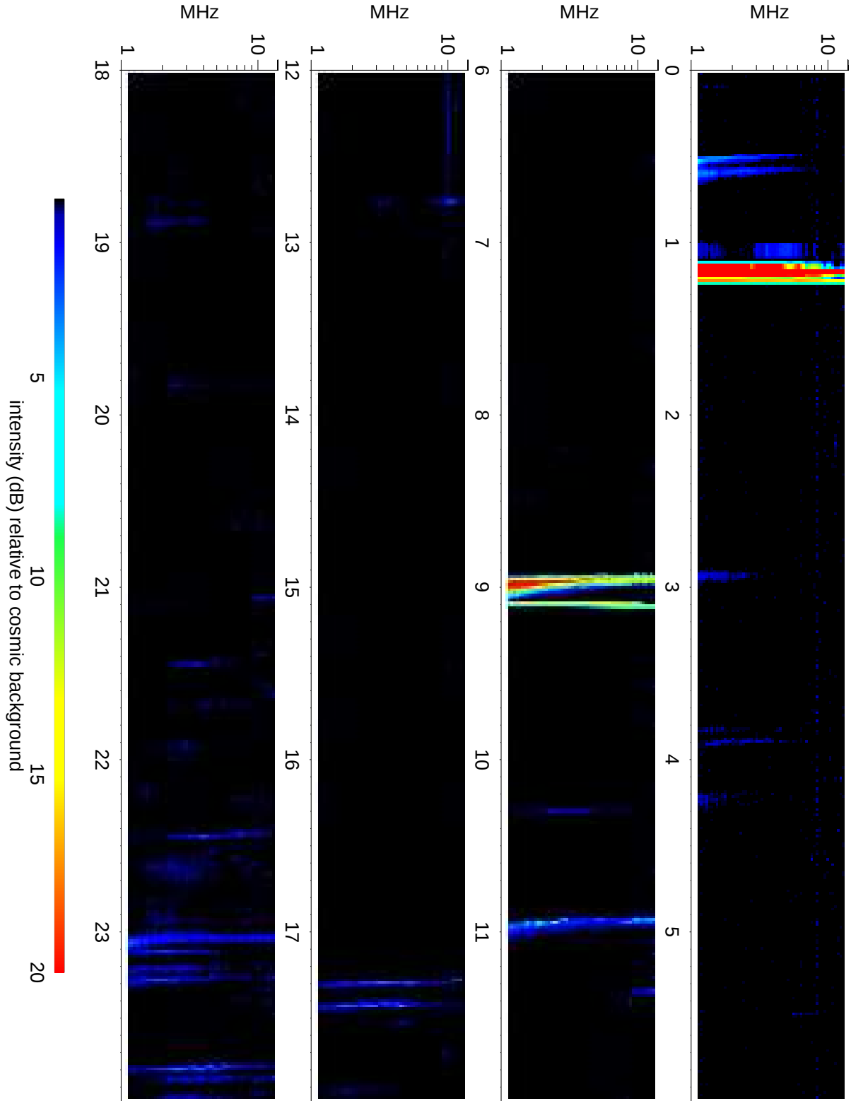
Wind Waves RAD2 receiver: 2010/10/17
