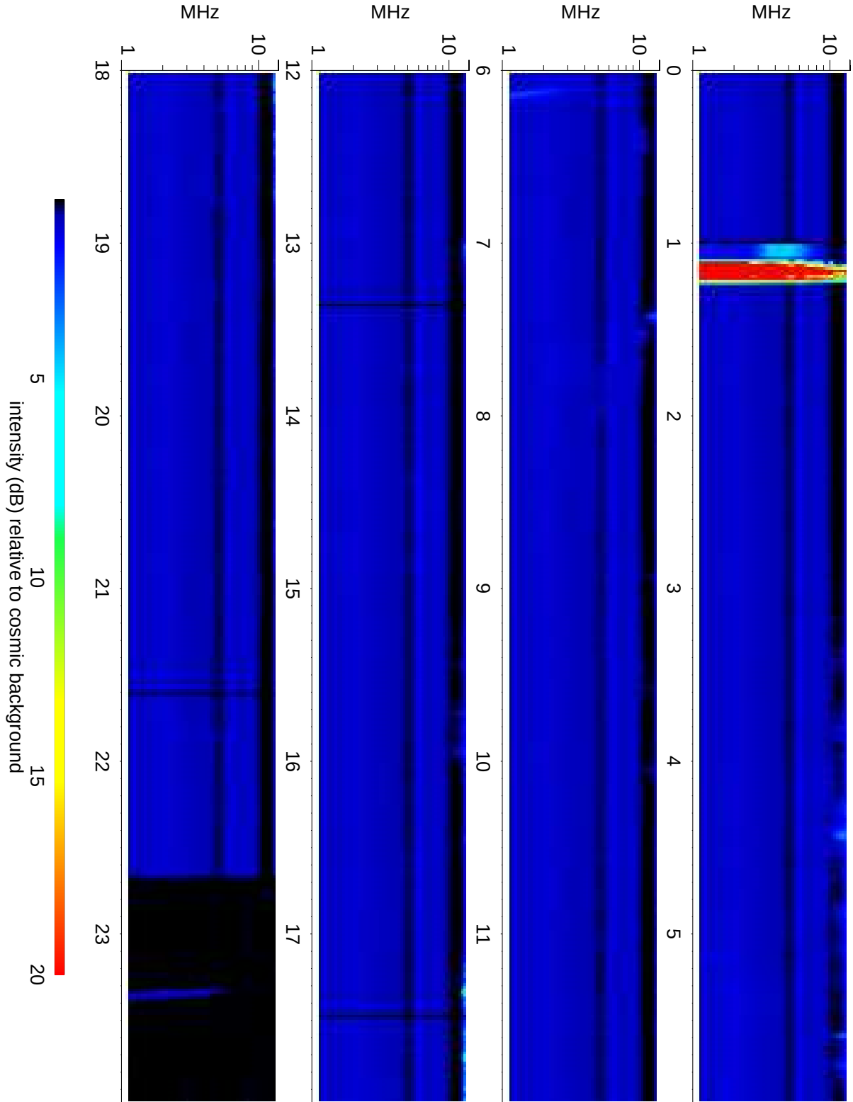
Wind Waves RAD2 receiver: 2010/11/04
