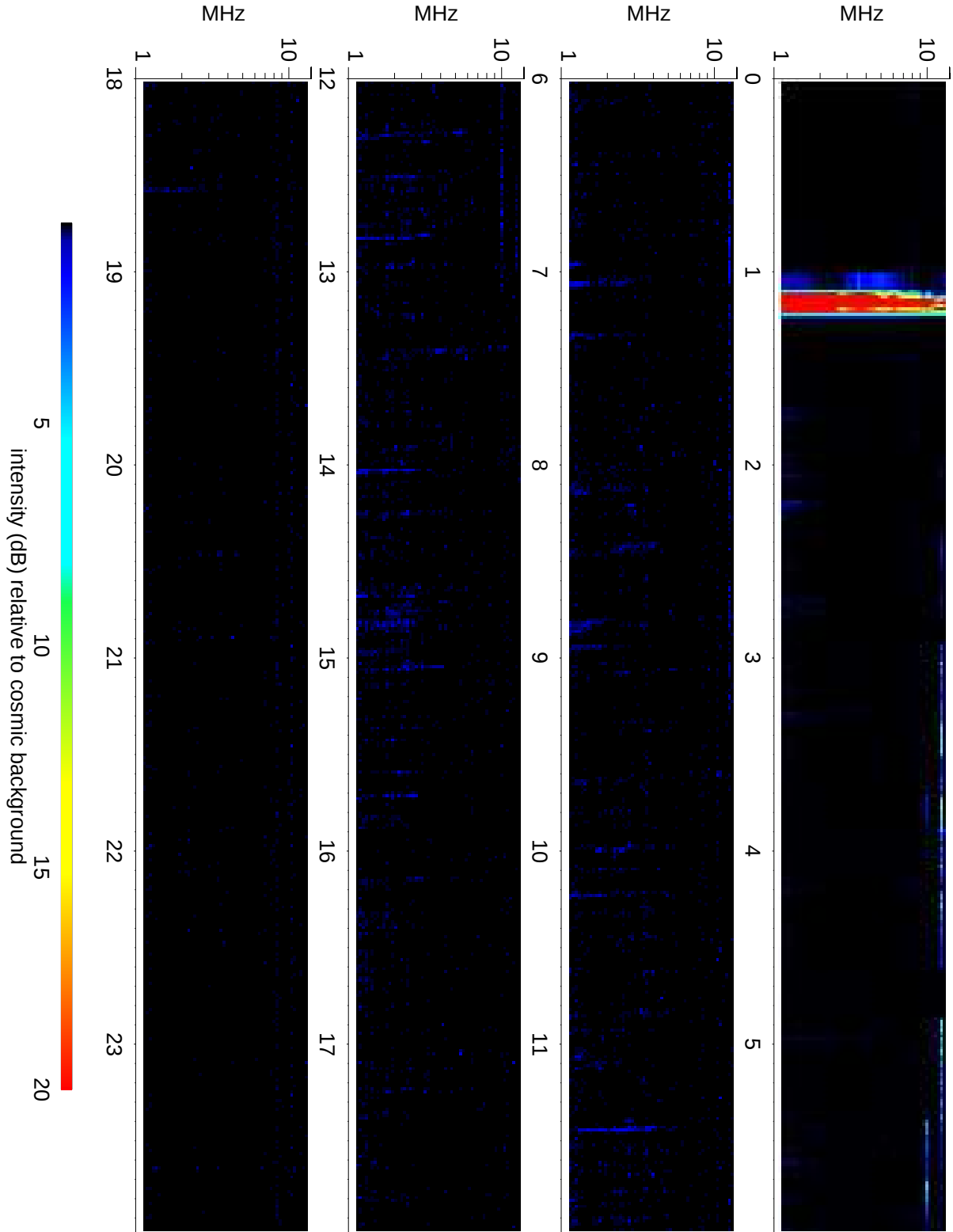
Wind Waves RAD2 receiver: 2010/11/20
