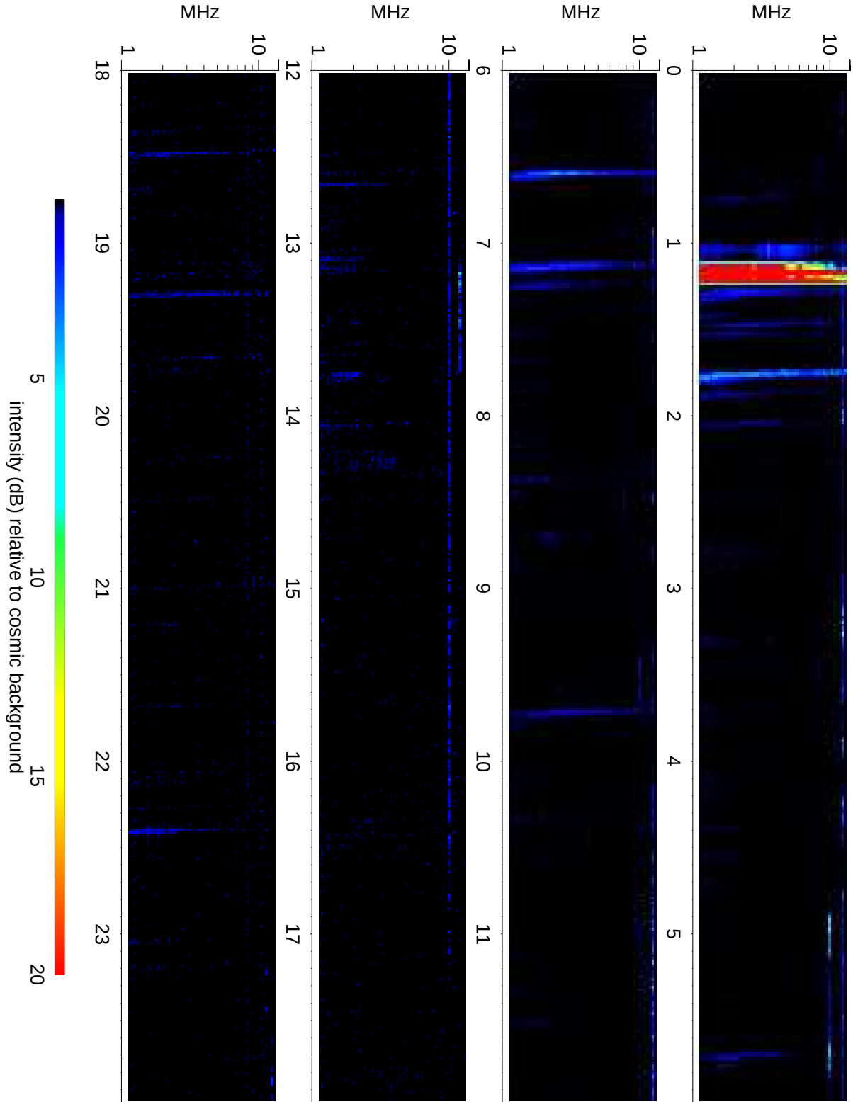
Wind Waves RAD2 receiver: 2010/12/10
