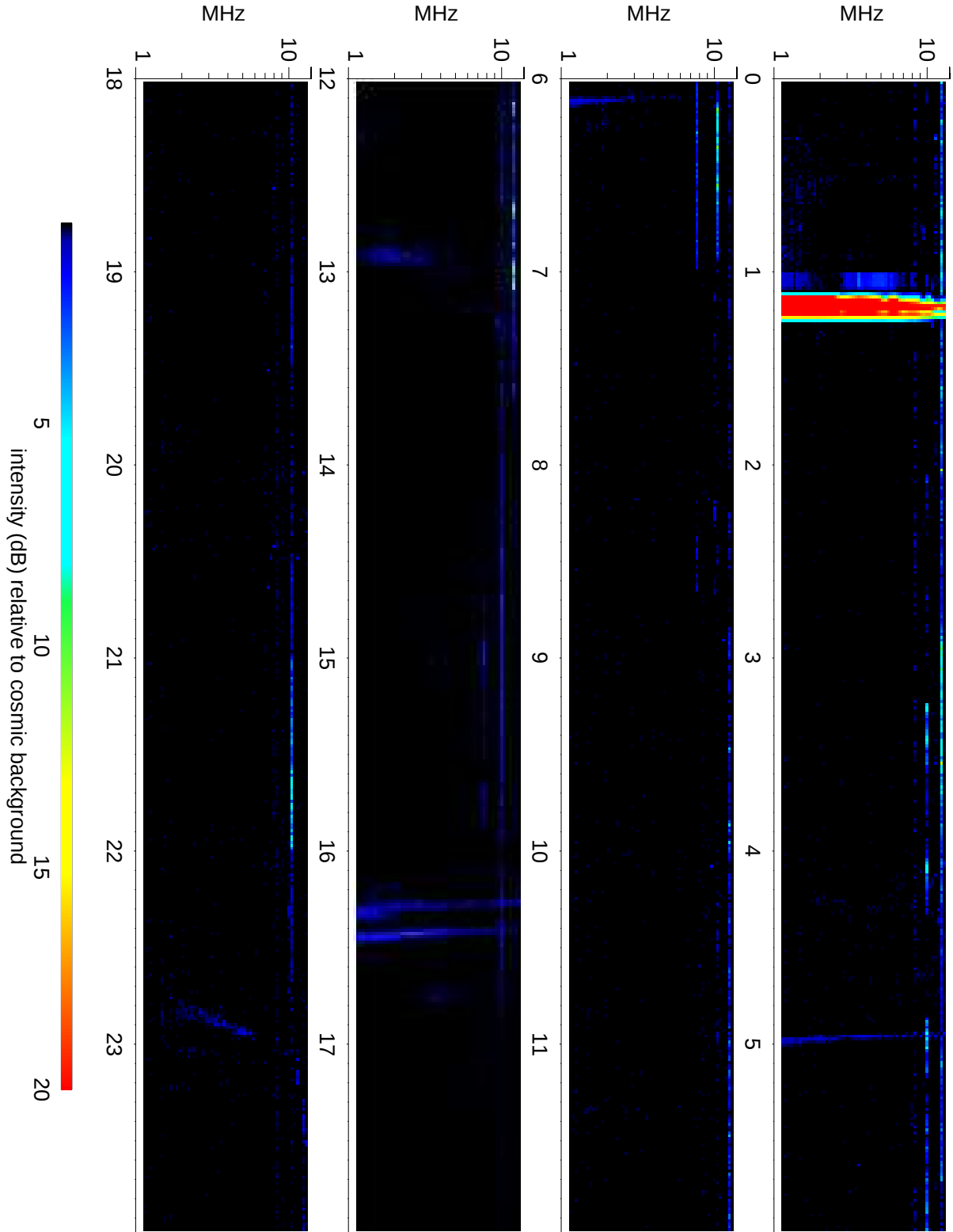
Wind Waves RAD2 receiver: 2010/12/30
