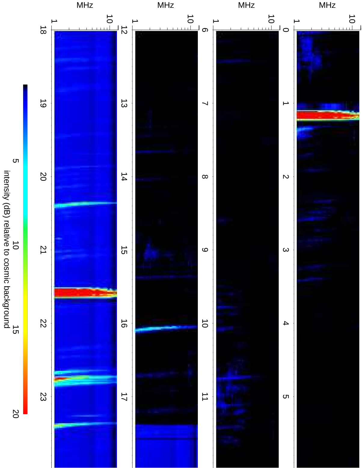
Wind Waves RAD2 receiver: 2012/10/24
