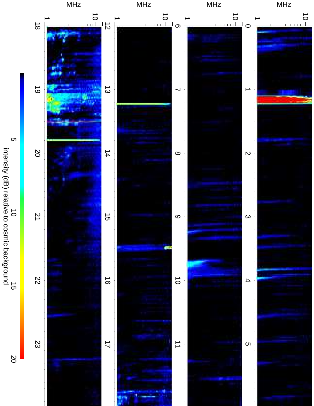
Wind Waves RAD2 receiver: 2014/01/04
