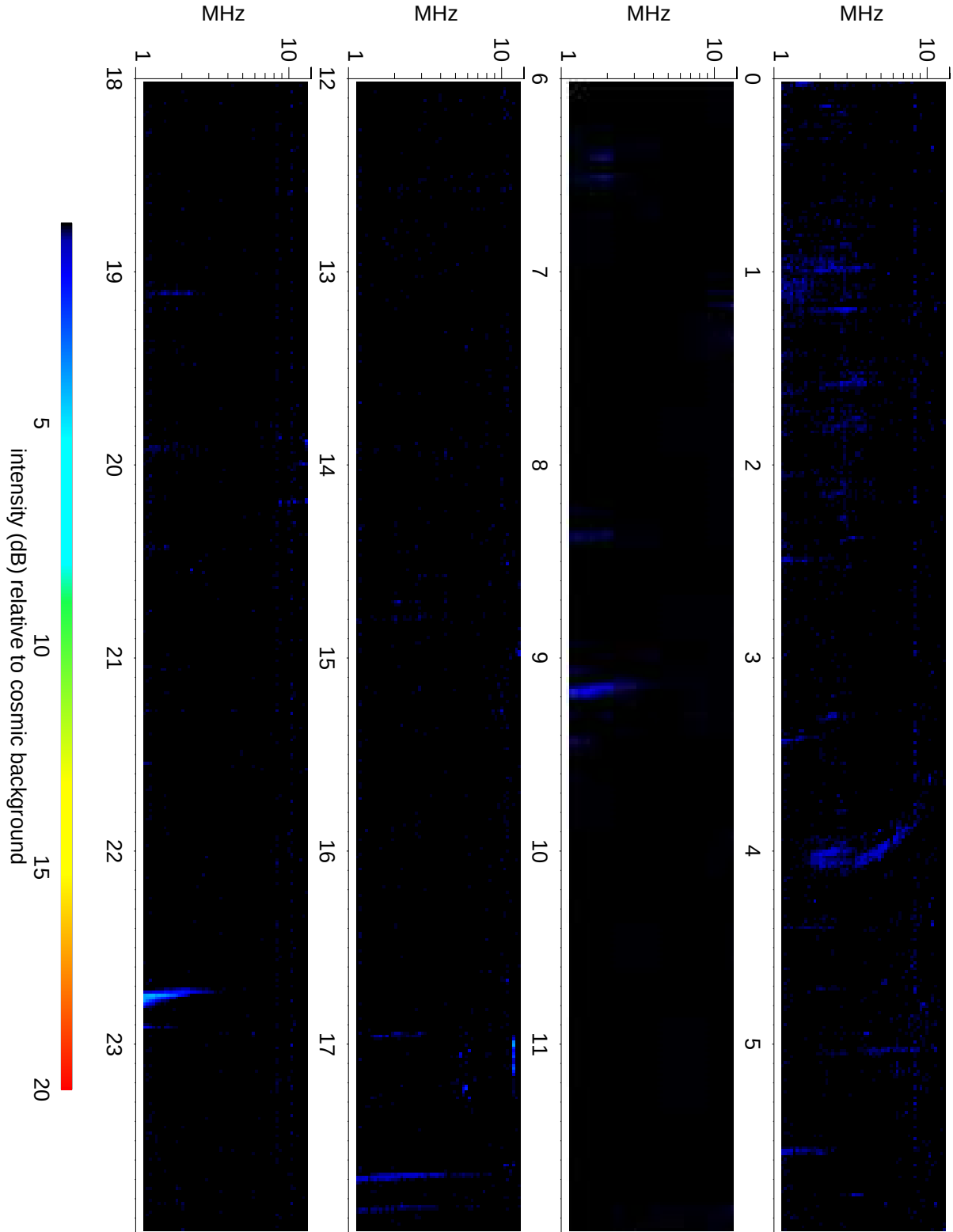
Wind Waves RAD2 receiver: 2014/01/11
