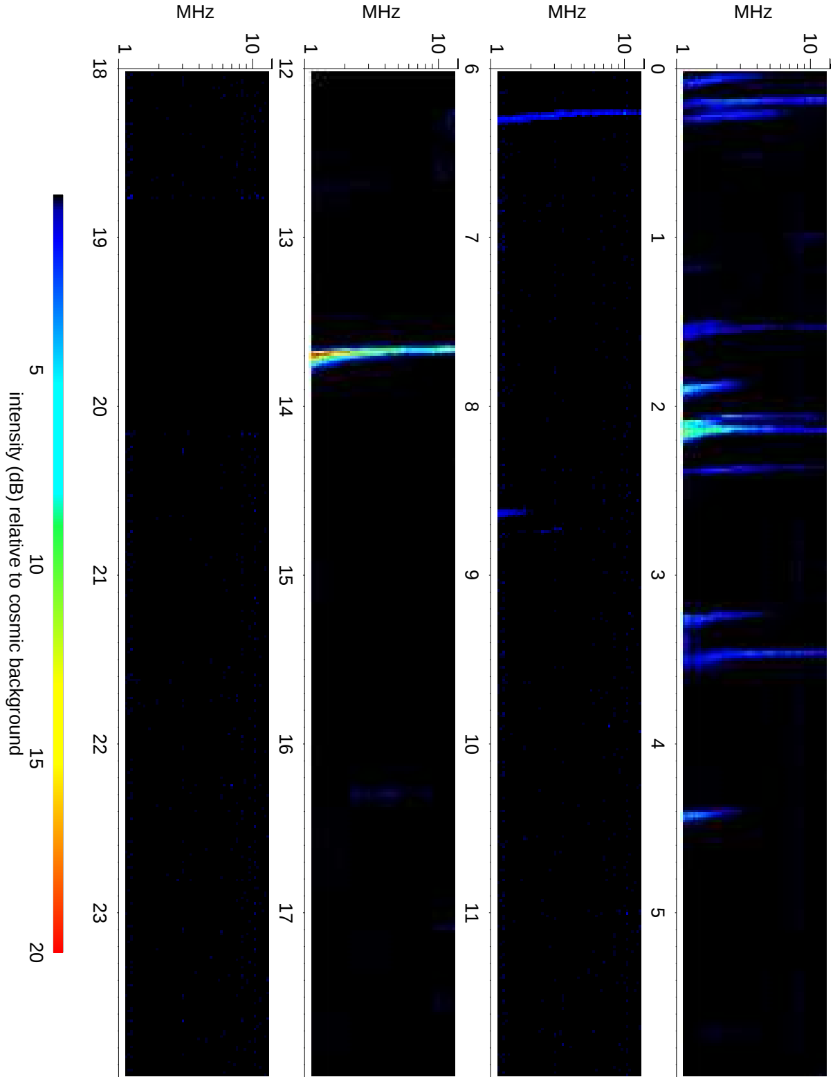
Wind Waves RAD2 receiver: 2014/03/16
