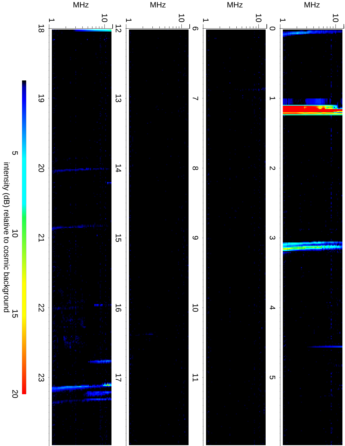
Wind Waves RAD2 receiver: 2014/04/10
