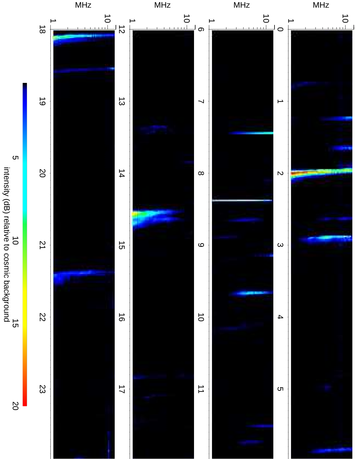
Wind Waves RAD2 receiver: 2014/04/11
