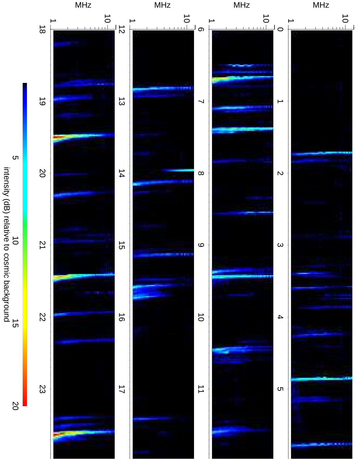
Wind Waves RAD2 receiver: 2014/04/19
