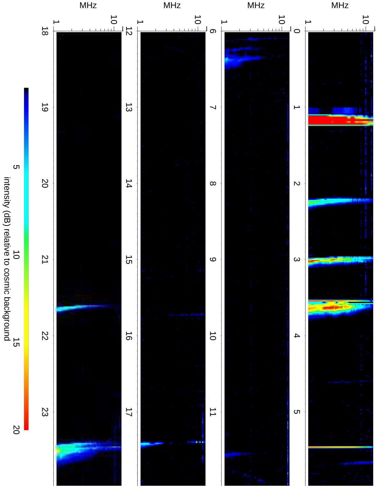
Wind Waves RAD2 receiver: 2014/05/28
