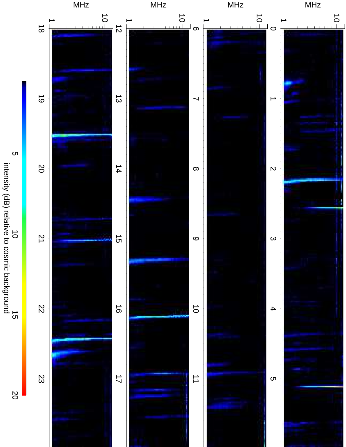
Wind Waves RAD2 receiver: 2014/06/06
