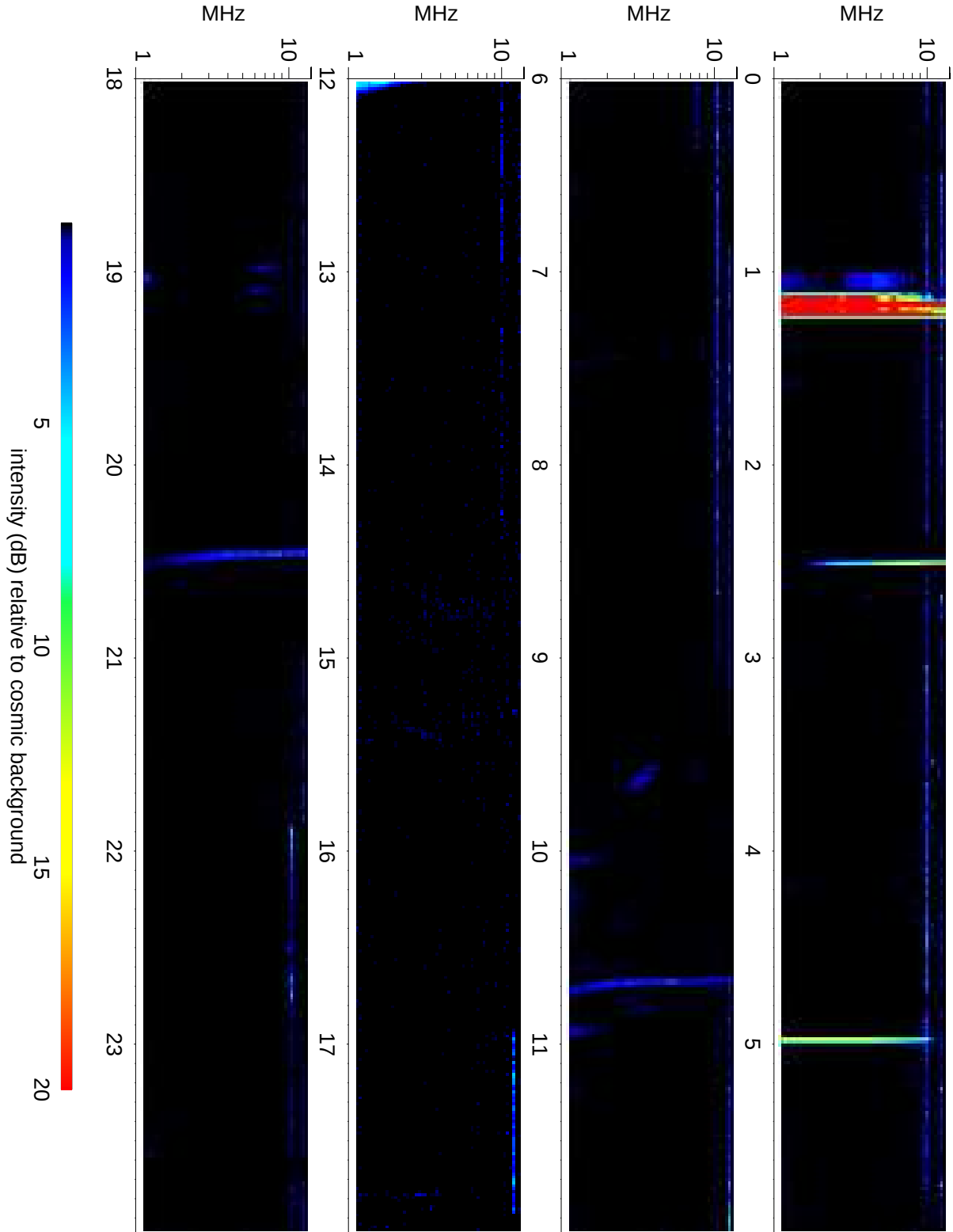
Wind Waves RAD2 receiver: 2014/06/19
