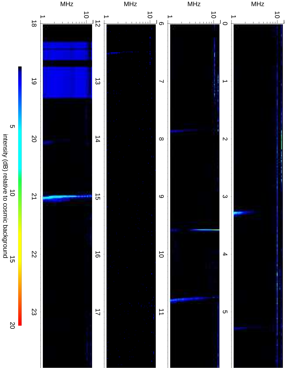
Wind Waves RAD2 receiver: 2014/06/24
