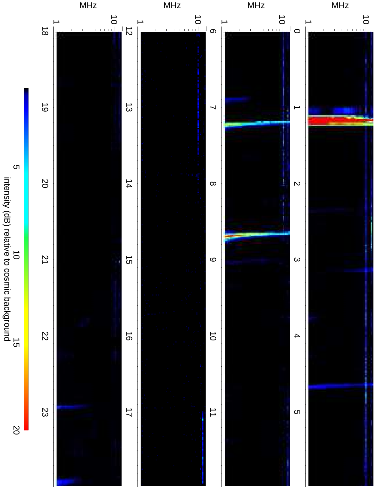
Wind Waves RAD2 receiver: 2014/06/25
