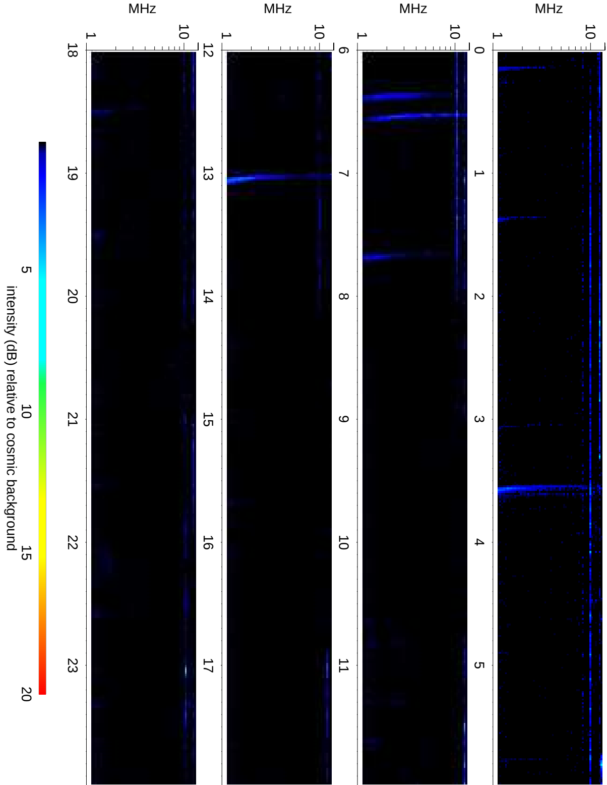
Wind Waves RAD2 receiver: 2014/06/28
