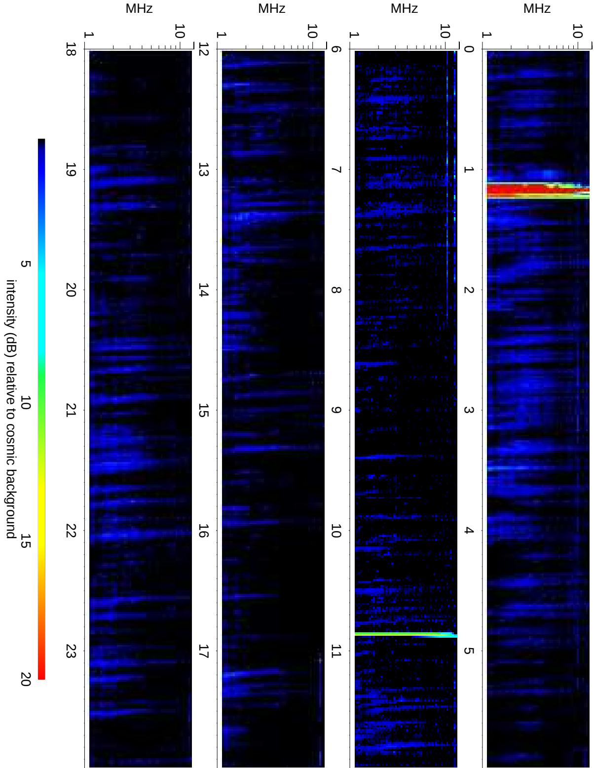
Wind Waves RAD2 receiver: 2014/07/03
