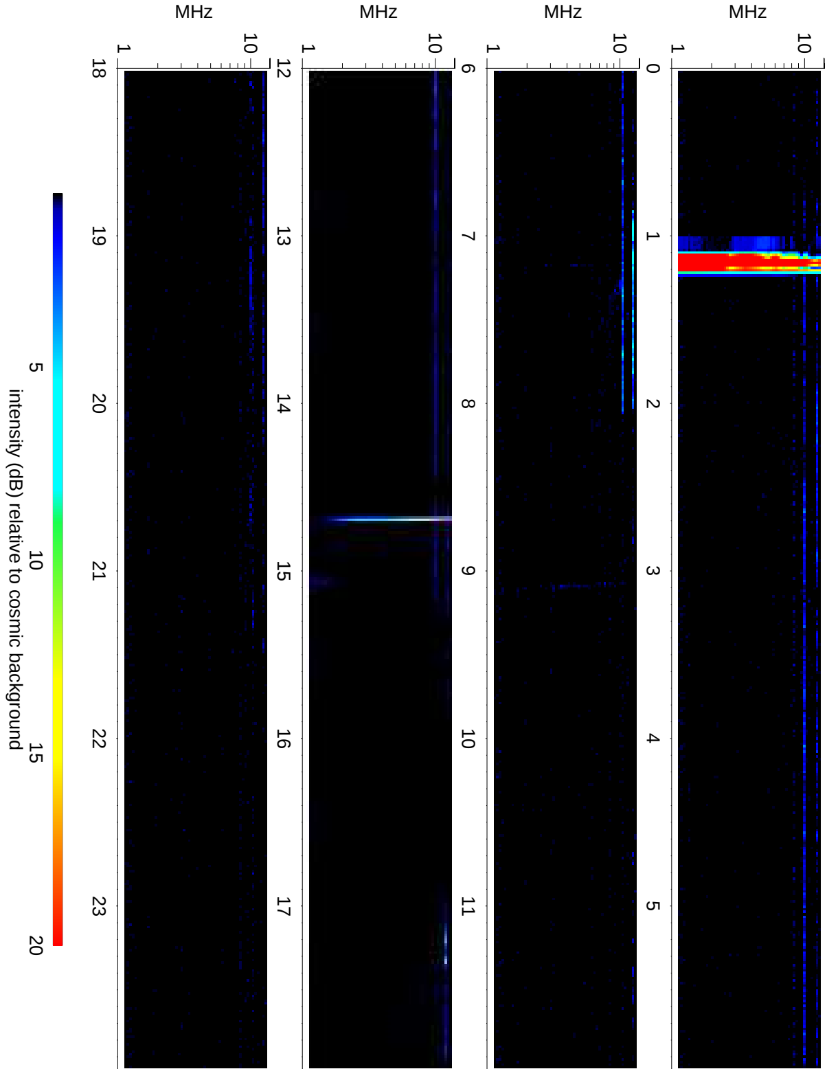
Wind Waves RAD2 receiver: 2014/07/15
