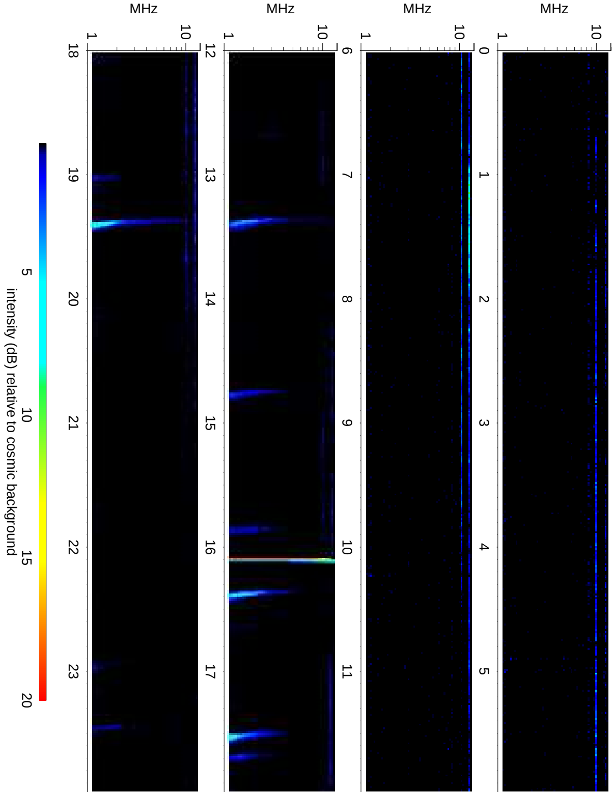
Wind Waves RAD2 receiver: 2014/07/20
