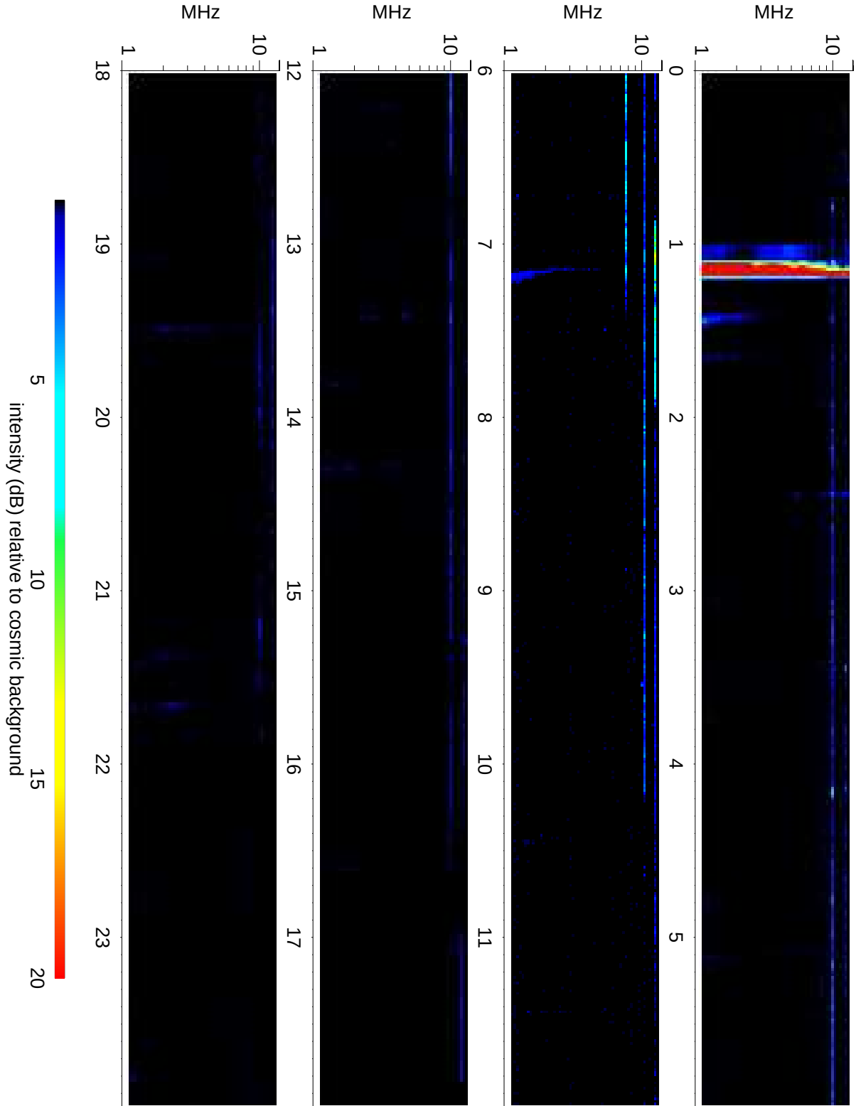
Wind Waves RAD2 receiver: 2014/07/21
