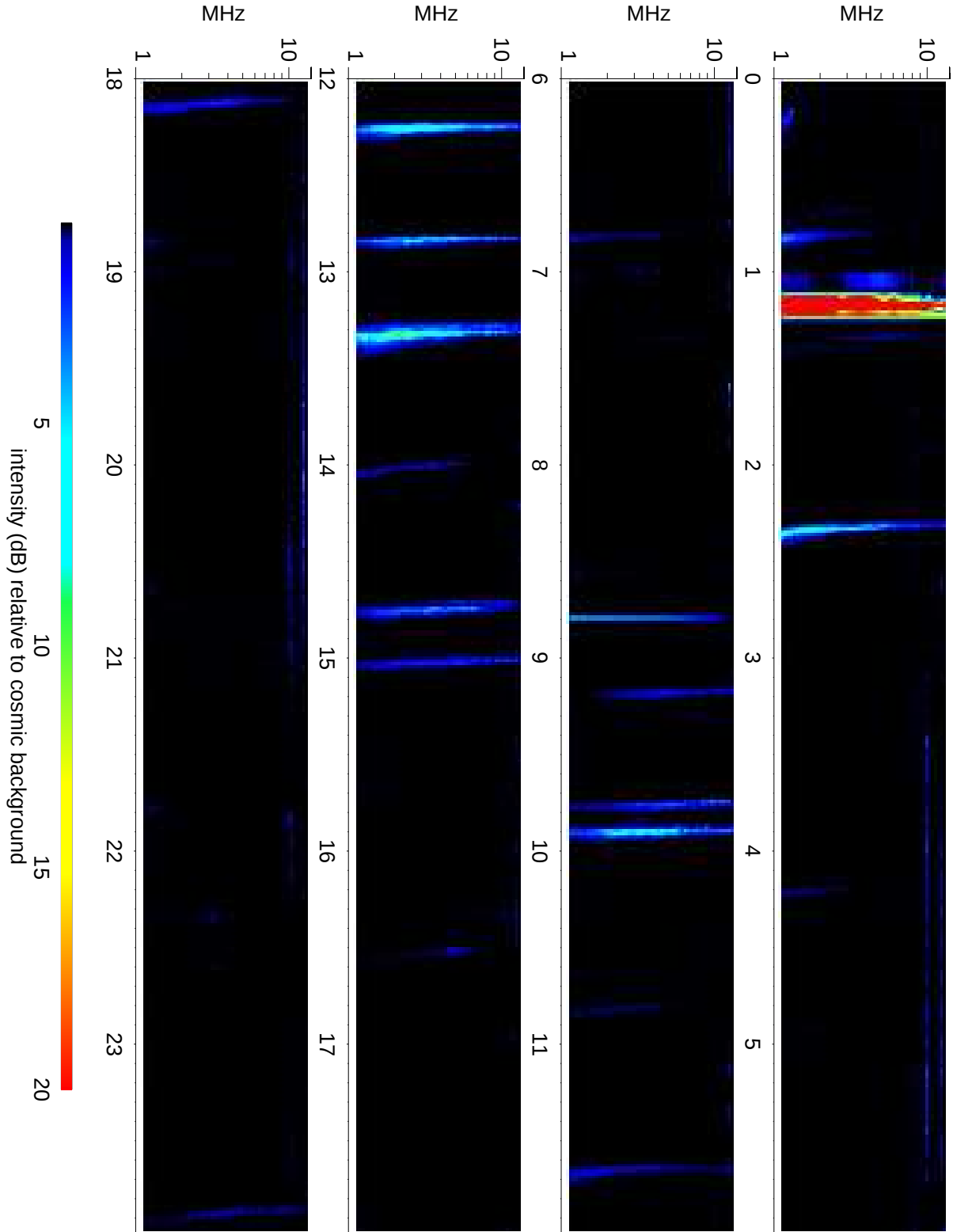
Wind Waves RAD2 receiver: 2014/08/02
