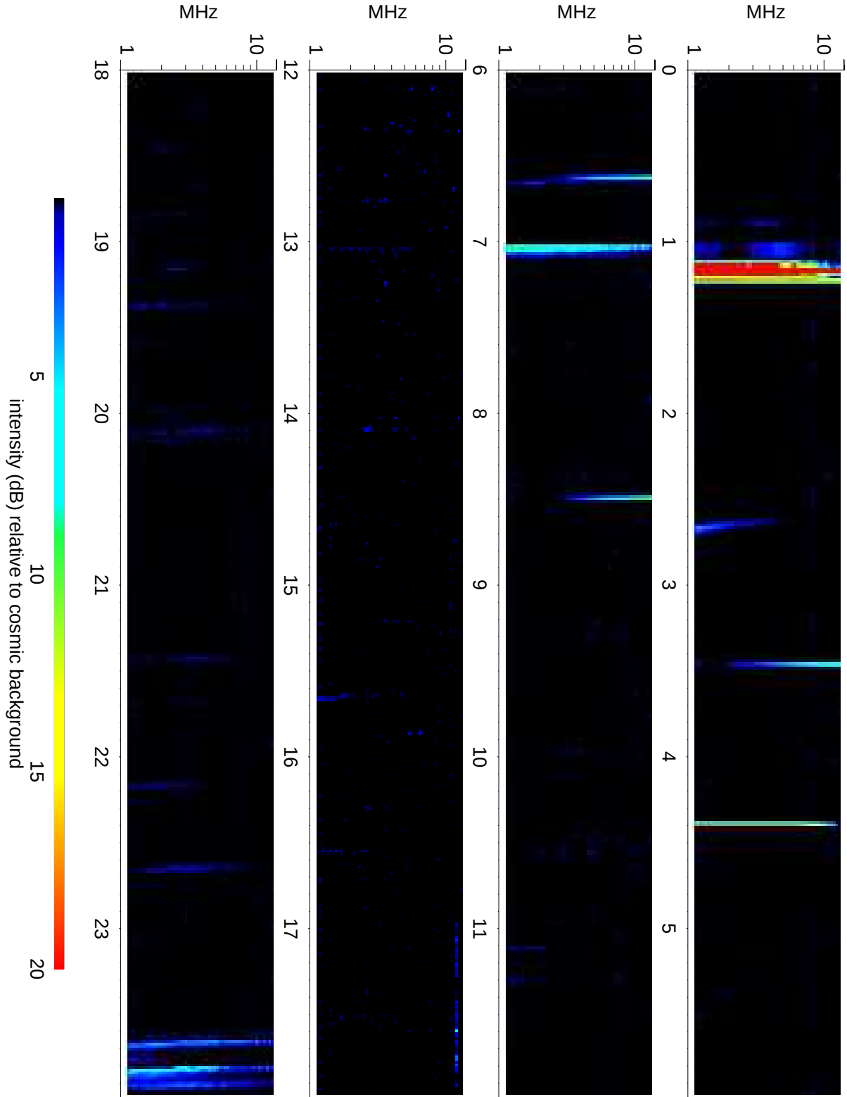
Wind Waves RAD2 receiver: 2014/09/11
