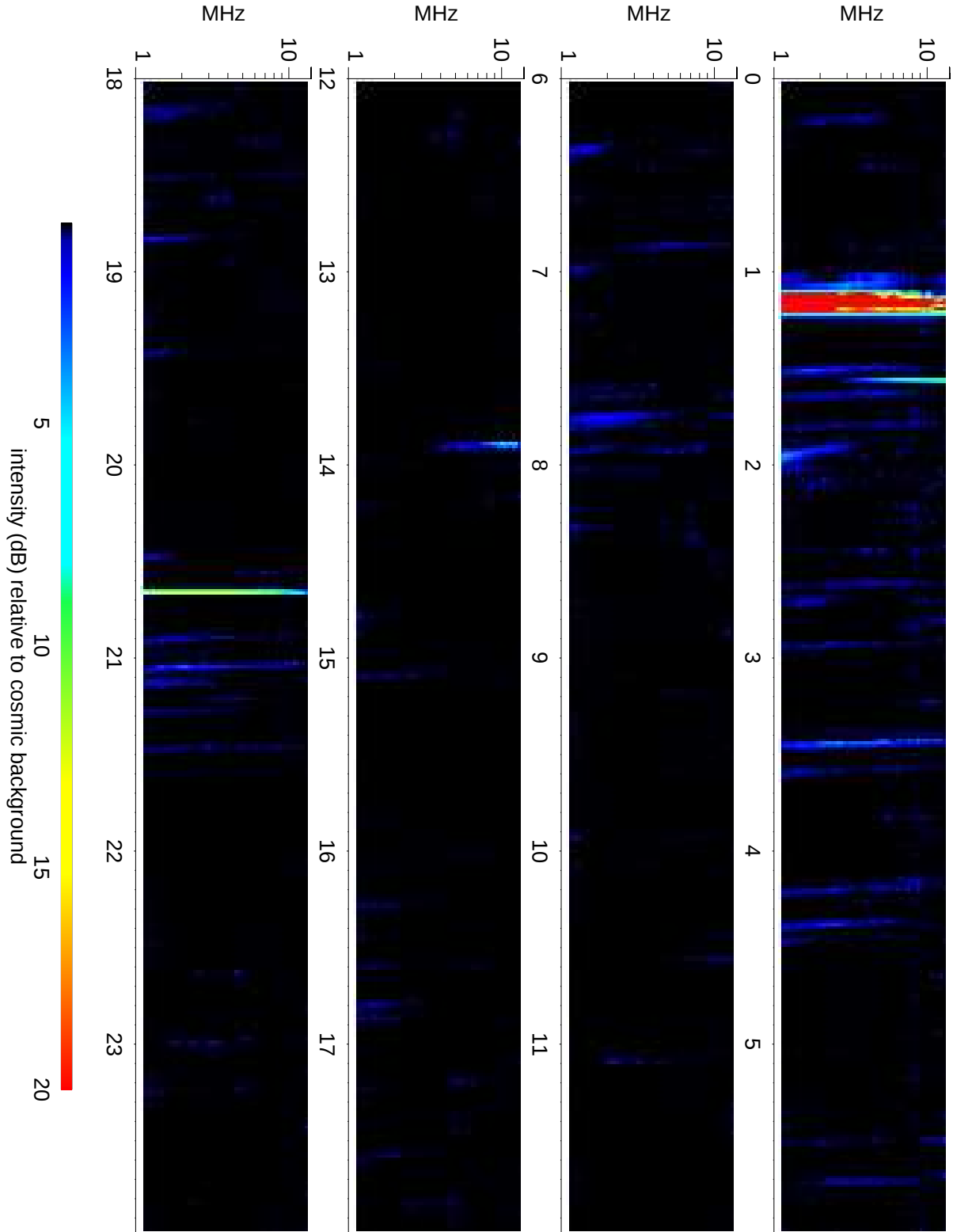
Wind Waves RAD2 receiver: 2014/10/15
