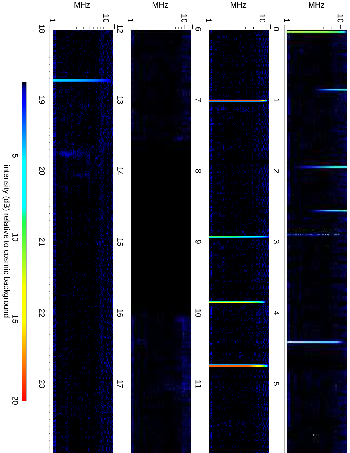
Wind Waves RAD2 receiver: 2014/11/23
