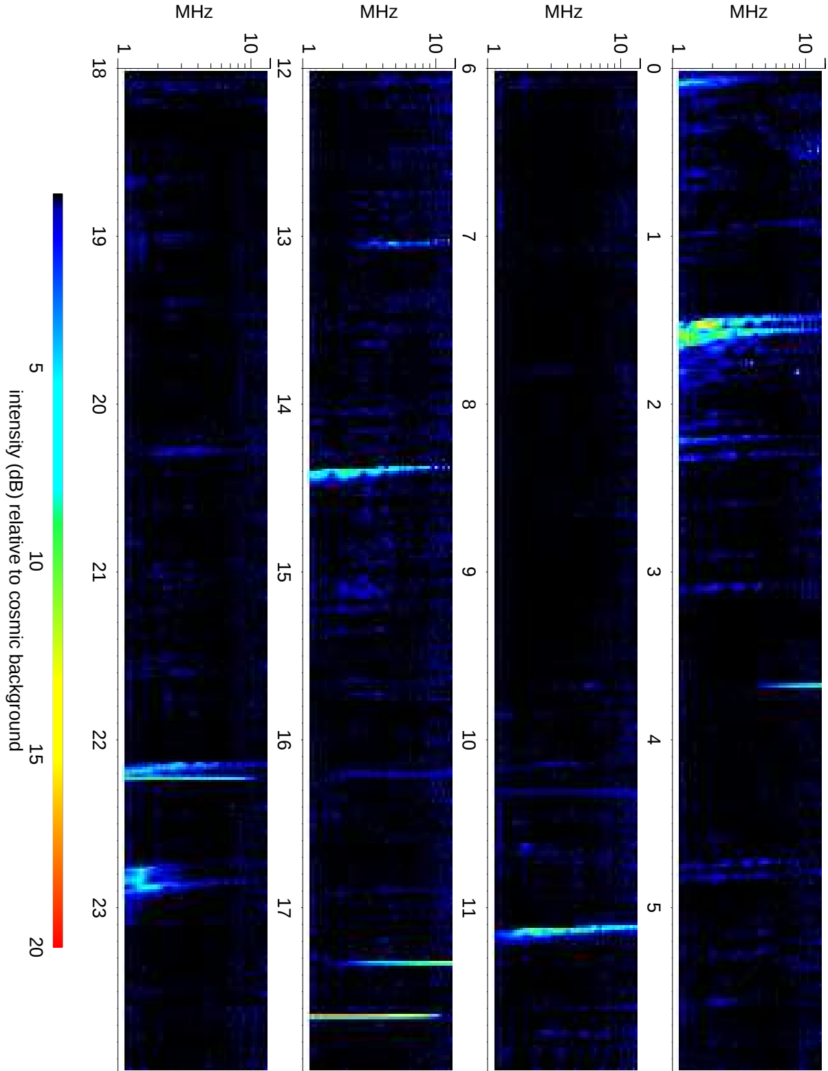
Wind Waves RAD2 receiver: 2014/11/29
