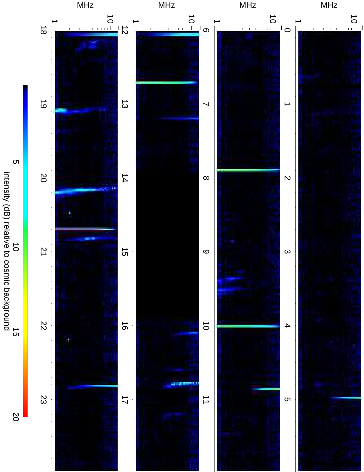
Wind Waves RAD2 receiver: 2014/12/01
