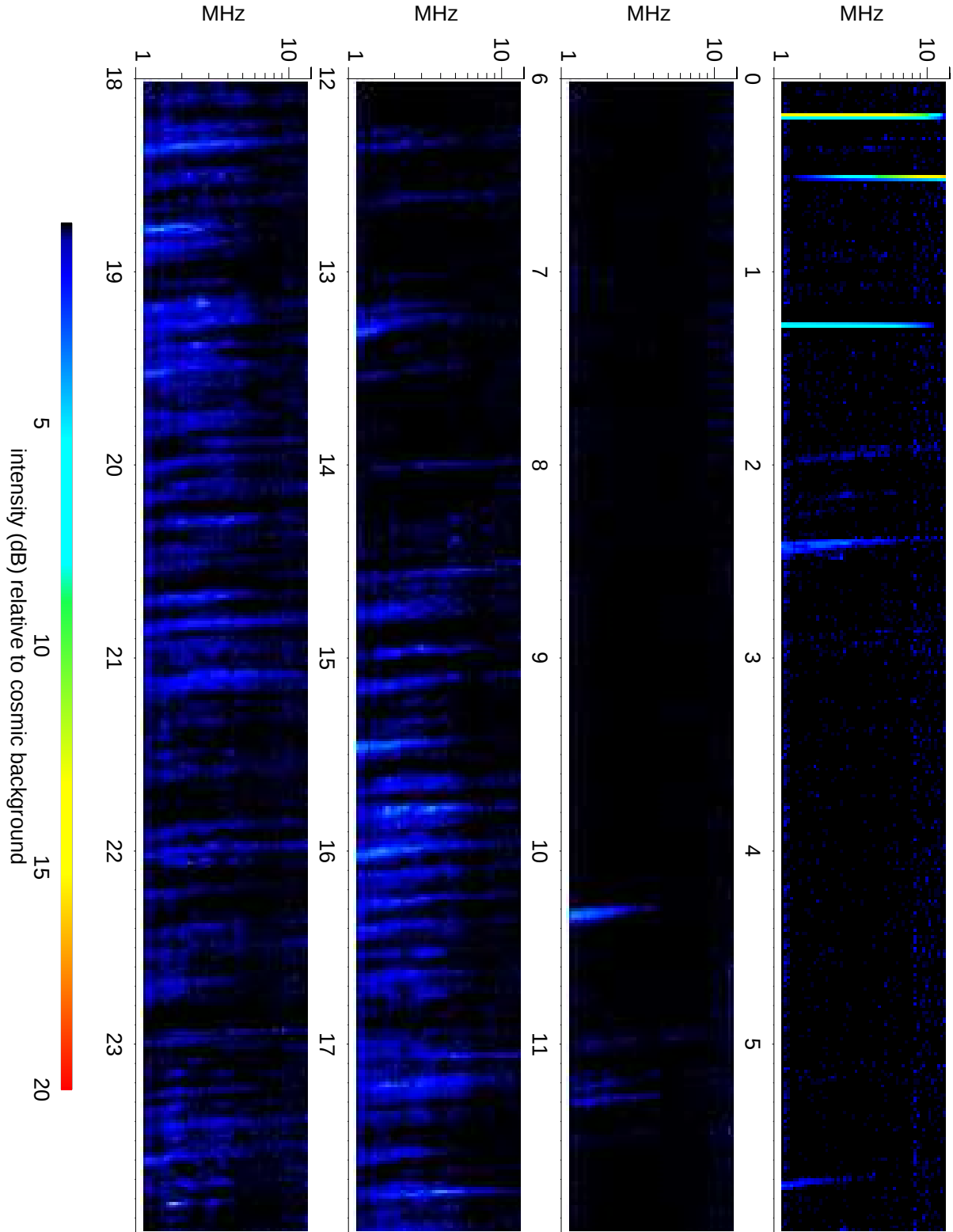
Wind Waves RAD2 receiver: 2014/12/04
