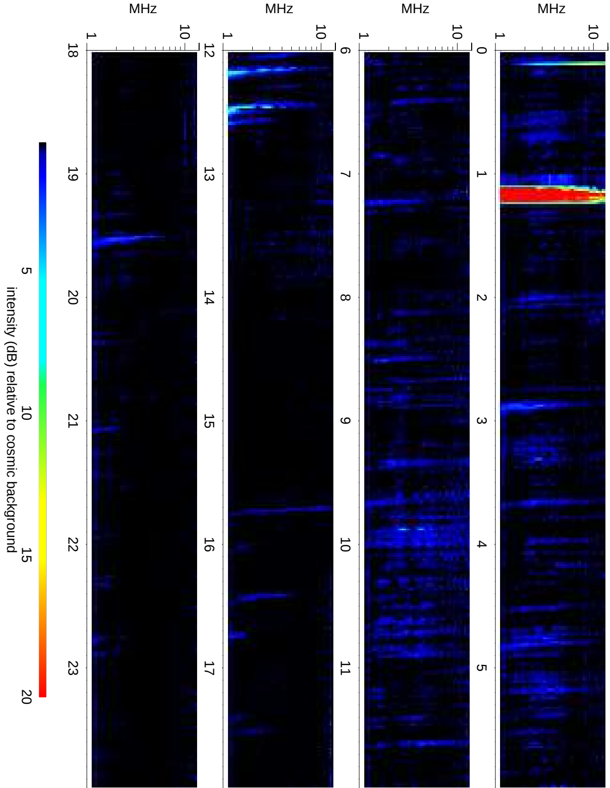
Wind Waves RAD2 receiver: 2014/12/06
