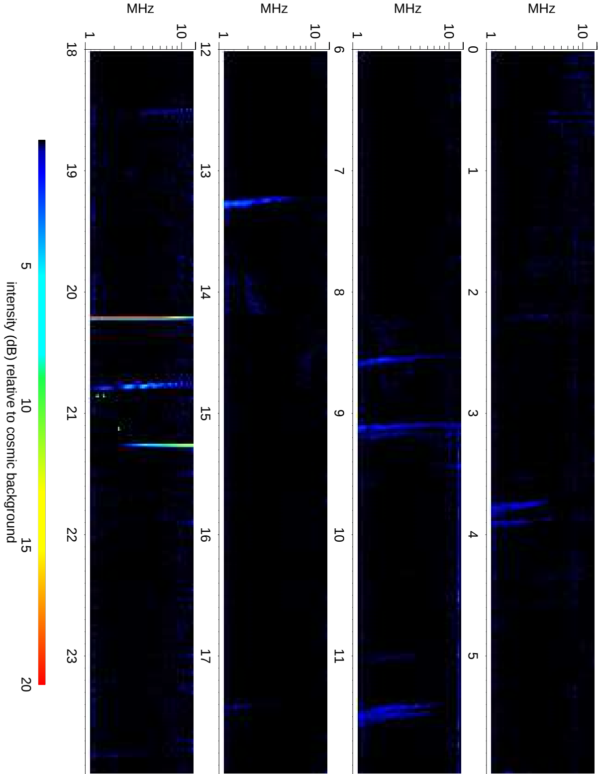
Wind Waves RAD2 receiver: 2014/12/11
