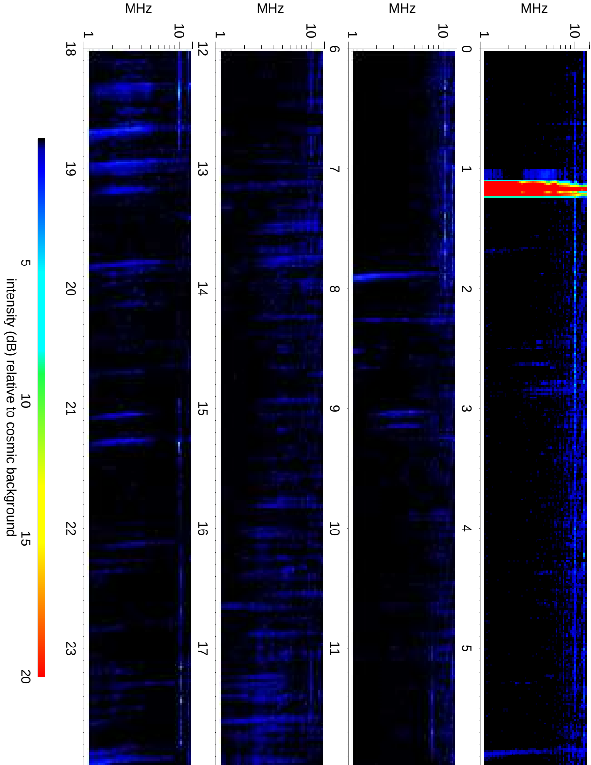
Wind Waves RAD2 receiver: 2015/06/23
