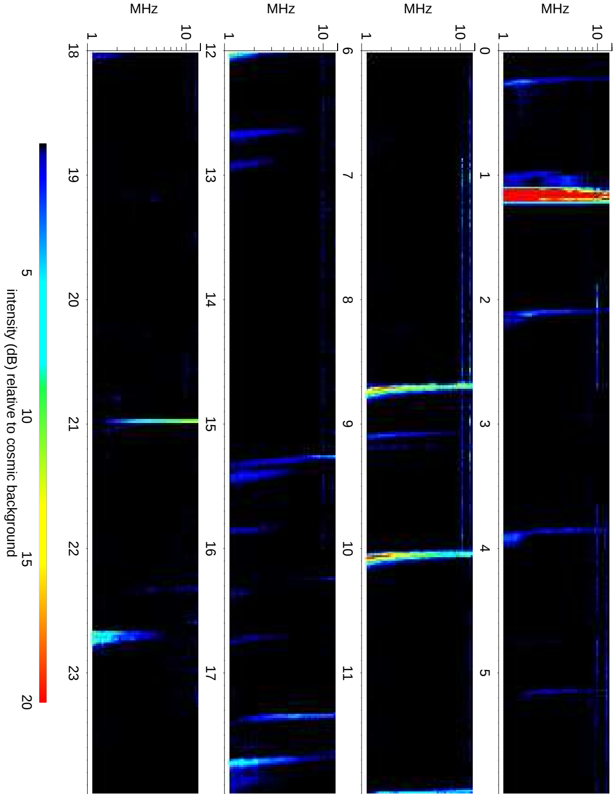
Wind Waves RAD2 receiver: 2015/08/02
