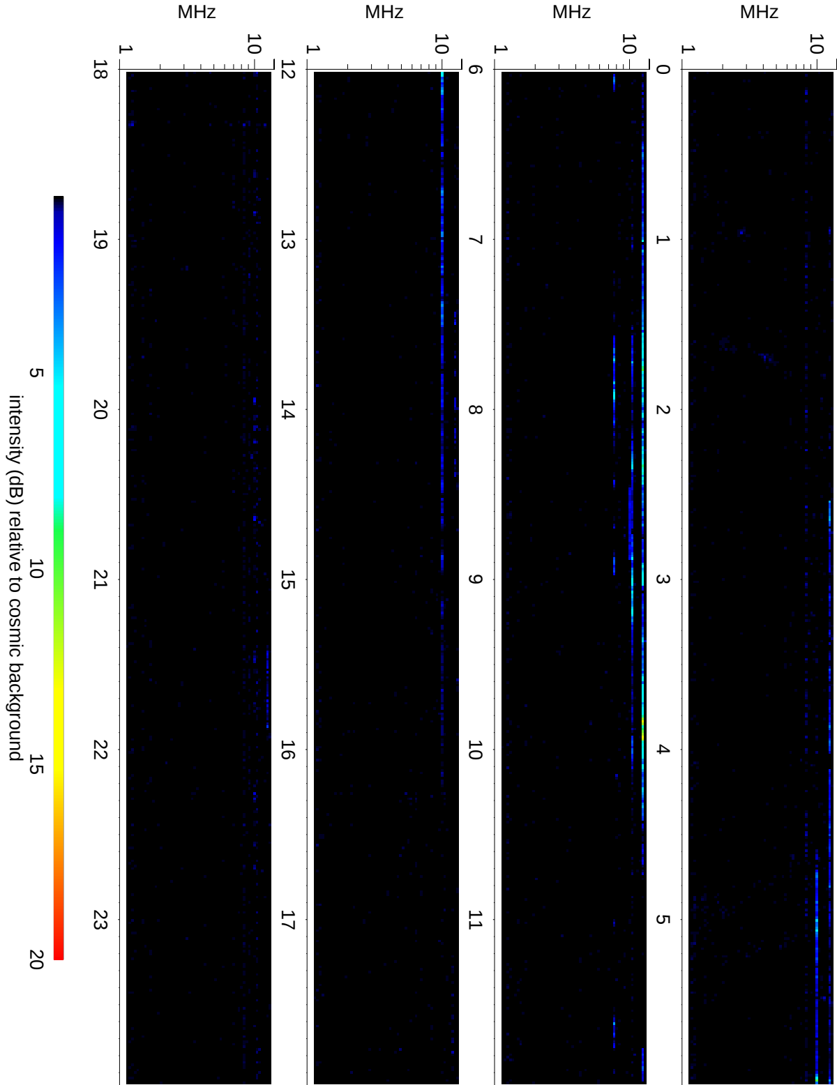
Wind Waves RAD2 receiver: 2018/01/27
