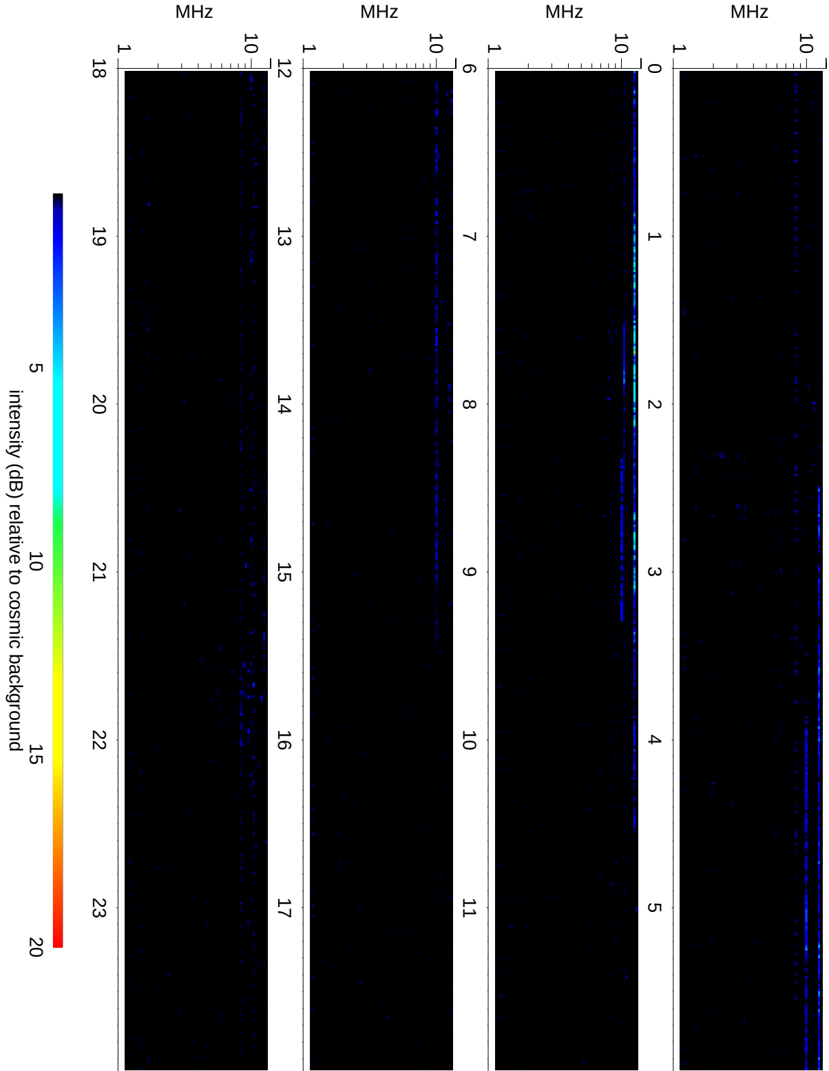
Wind Waves RAD2 receiver: 2018/02/18
