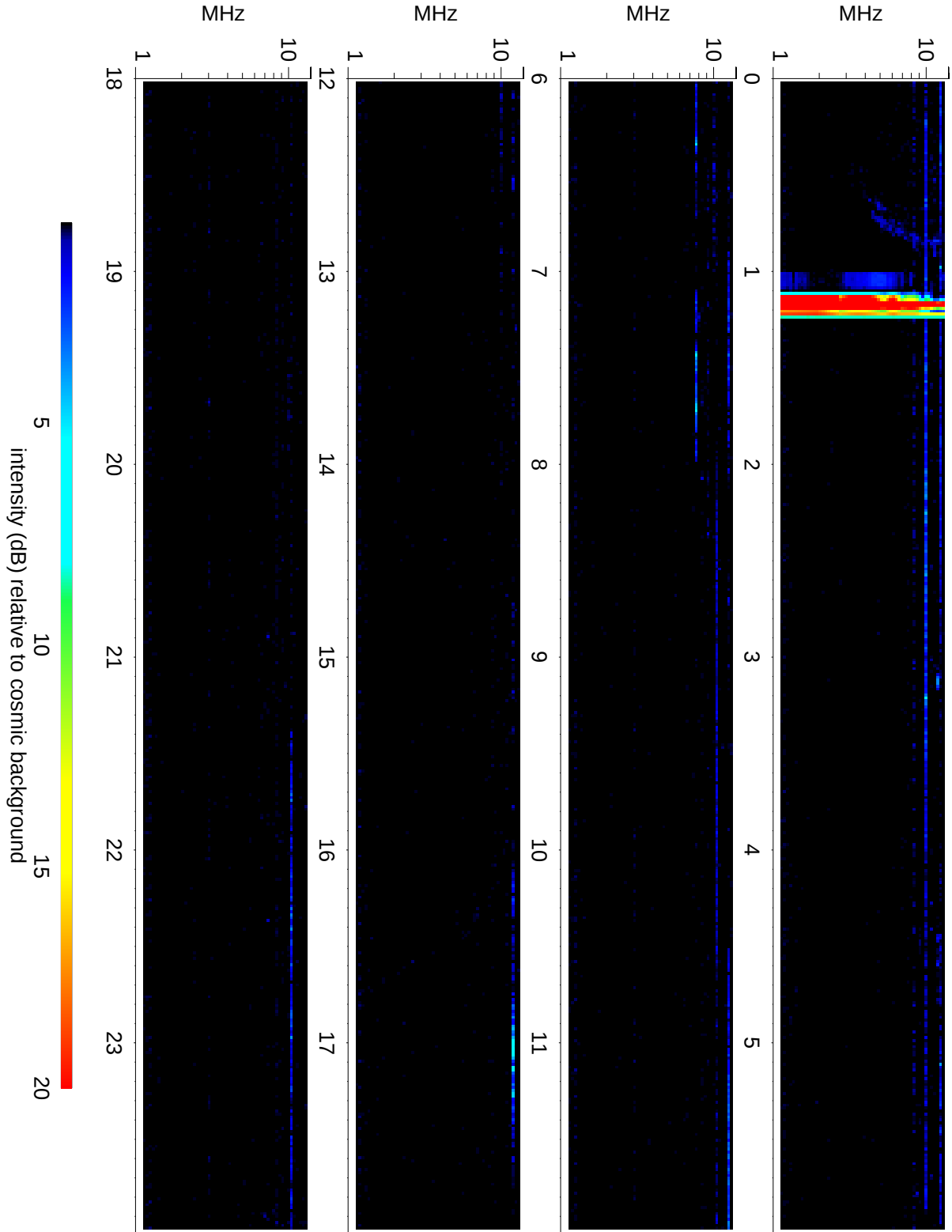
Wind Waves RAD2 receiver: 2018/04/12
